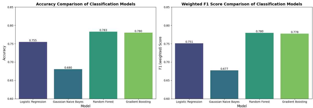
Figure 7. Classification Model Performance Comparison
