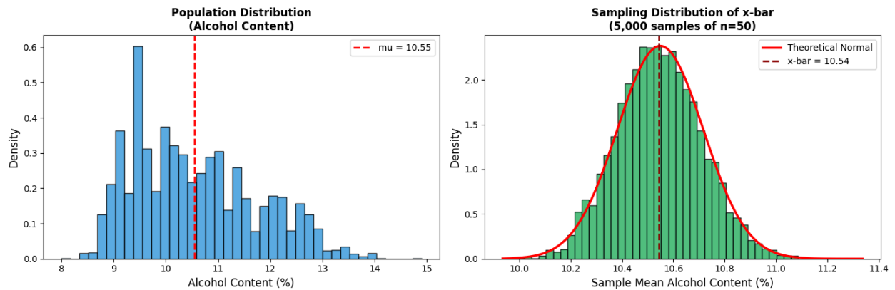
Figure 2. Central Limit Theorem: Population vs Sampling Distribution
